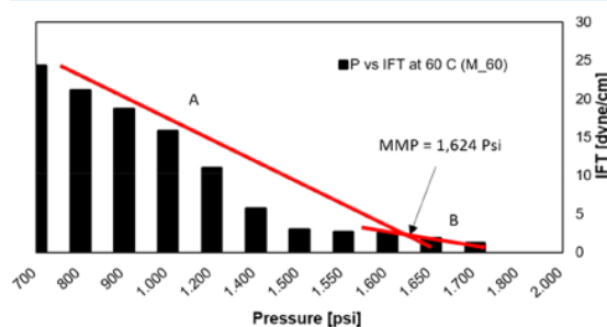
Figure 4. MMP from IFT test at T = 60 °C.
