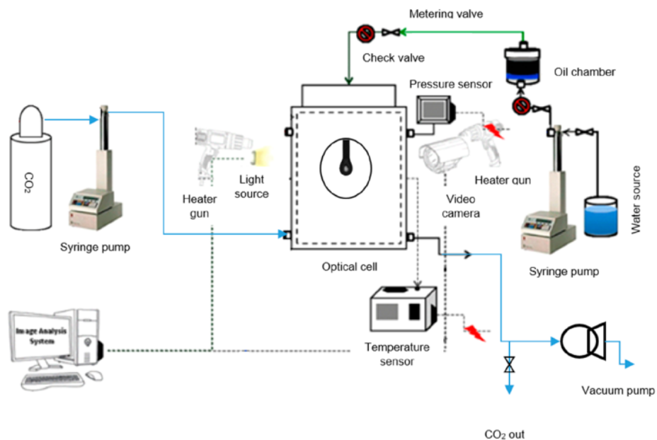
Figure 2. IFT experimental diagram. 26
