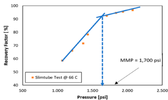
Figure 7. MMP from the slim-tube tests at T = 66\text{ }^{\circ}\text{C} .
