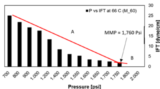
Figure 5. MMP from IFT test at T = 66 °C.
