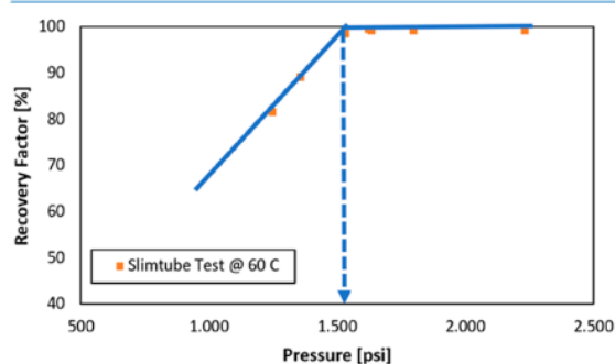
Figure 6. MMP from the slim-tube tests at T = 60 °C.
