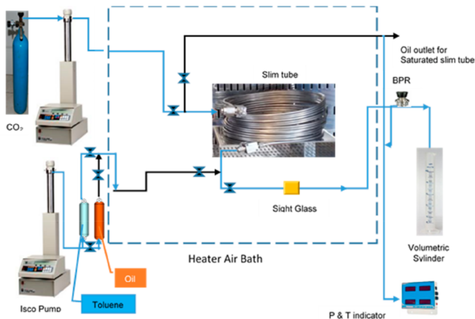
Figure 3. Slim tube test experimental diagram. 26
