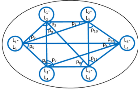
Figure 3. Bilingual Dictionary Induction Dependency Model.
