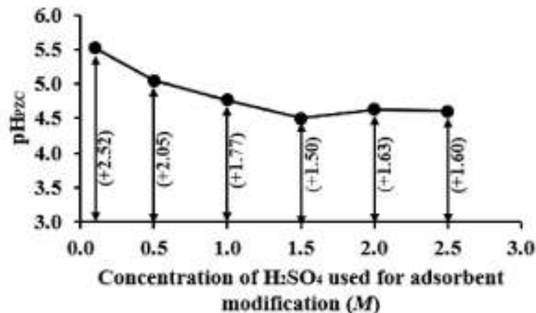
Figure 2. The point of zero charge (pH zpc ) values of various acid-modified sugarcane-bagasse-based adsorbents. The values in parentheses indicate the positivity of pH zpc subtracted by pH 3, i.e., the pH of the adsorption medium.
